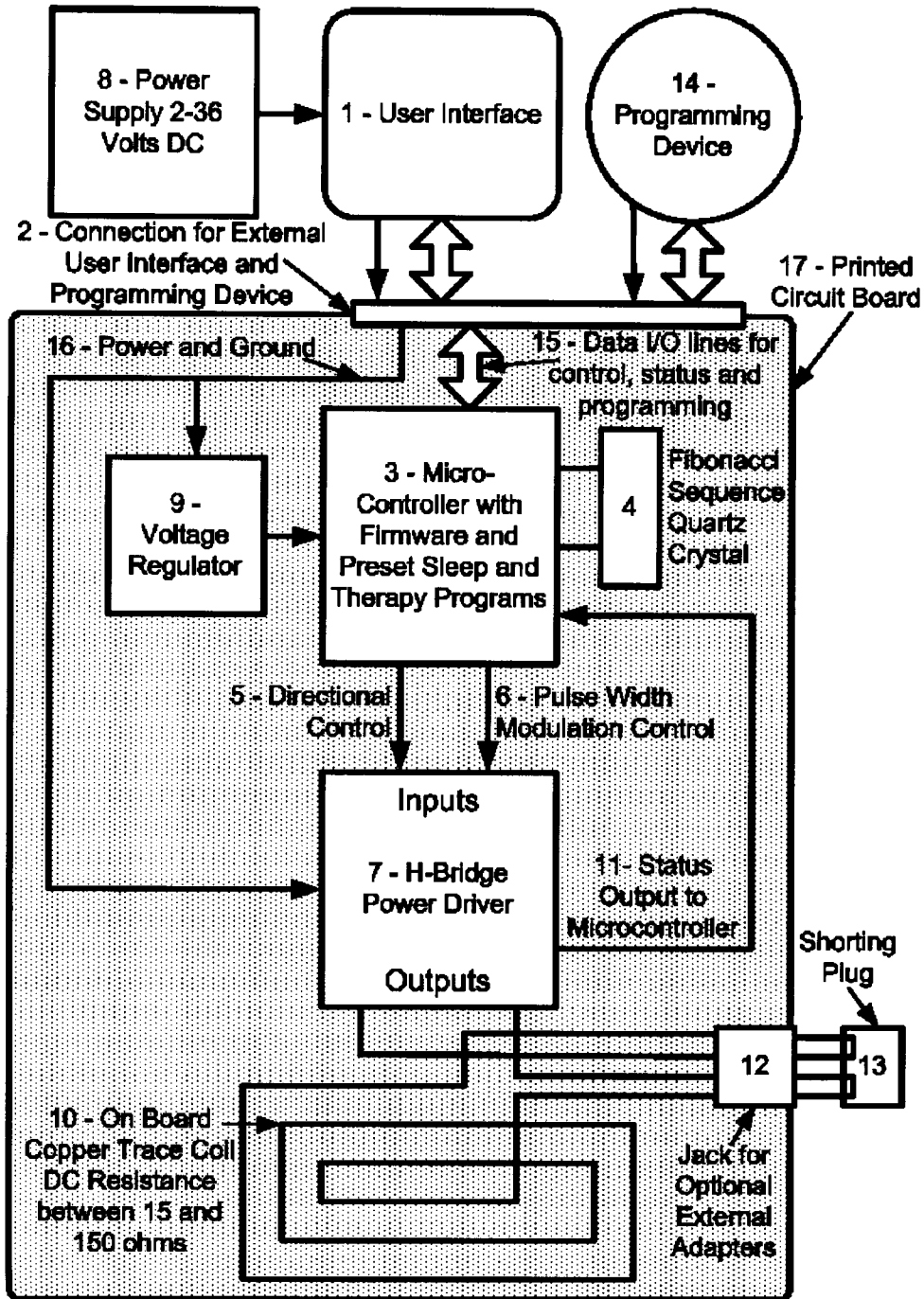
Block Diagram of EnergyWave Therapy Device
